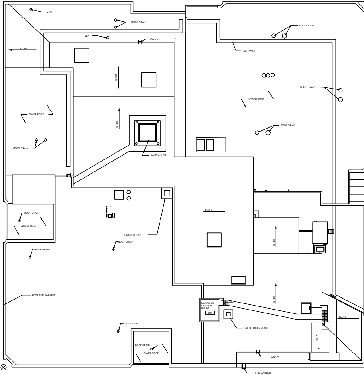
ROOF PLAN
