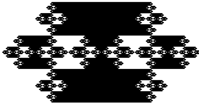
FIGURE 3. Lattice-tile for A = \begin{pmatrix} 3 & 0 \\ 0 & 3 \end{pmatrix} and \mathcal{D} = \{(-1, -1), (0, -1), (1, -1), (-2, 0), (0, 0), (2, 0), (-1, 1), (0, 1), (1, 1)\} .
