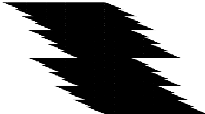
FIGURE 2. Lattice-tile for A = \begin{pmatrix} 2 & 1 \\ 0 & 2 \end{pmatrix} and \mathcal{D} = \{(0, 0), (1, 0), (0, 1), (1, 1)\} .
