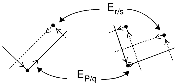
Fig. 1. The diamond conjecture.
