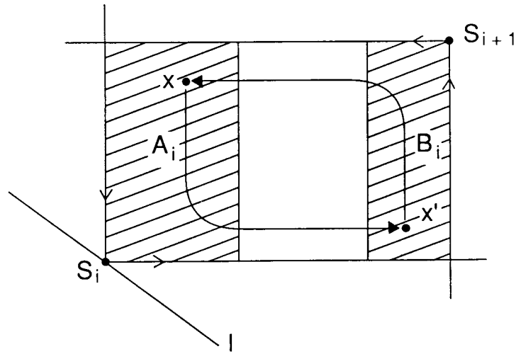
Fig. 2. The action of the R . The unshaded region is mapped outside K .
