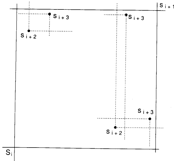
Fig. 6. The nested renormalization construction.
