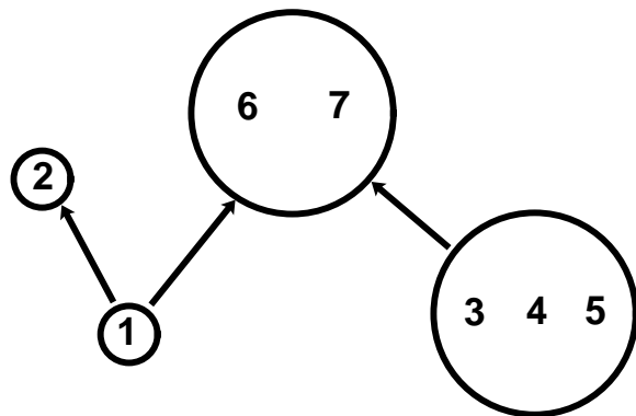
FIG. II.2. The condensation SC[G] of G in Figure II.1.
