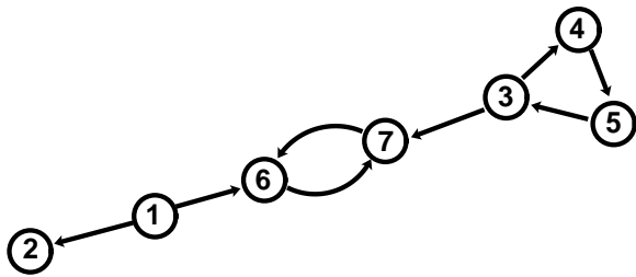
FIG. II.1. This graph will serve as an example throughout the paper.
