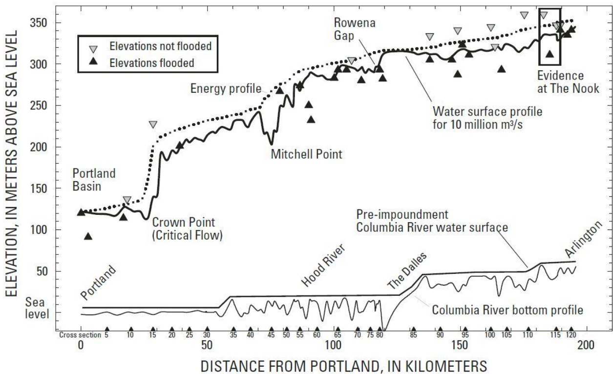
Figure 6. Evidence for maximum Missoula flood stages in lower Columbia River valley and step-backwater flow calculation results for a discharge of 10 million m 3 /s. Modified from Benito and O'Connor (2003).
