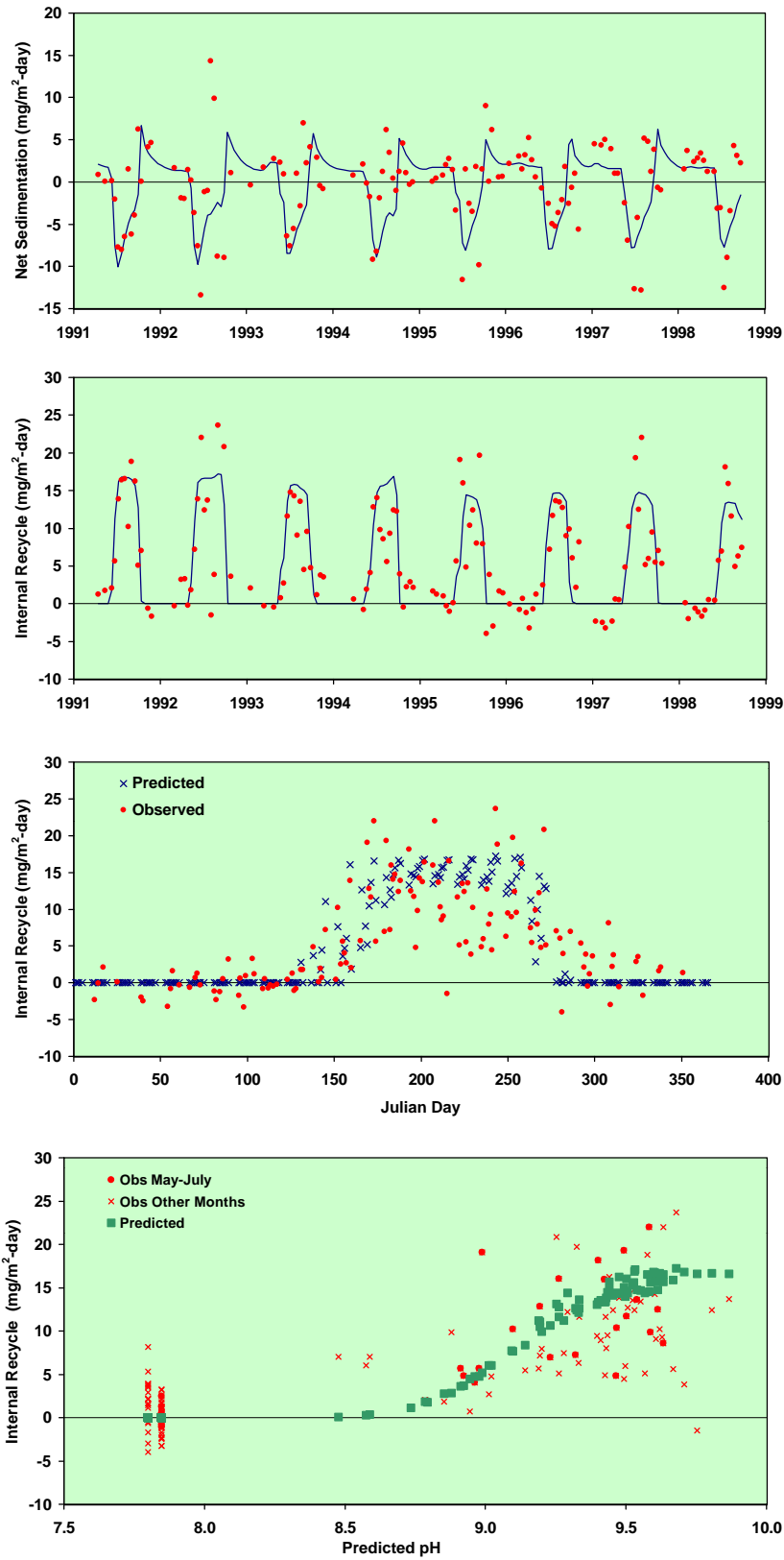
Figure 18 Calibration of Internal Recycle Function
