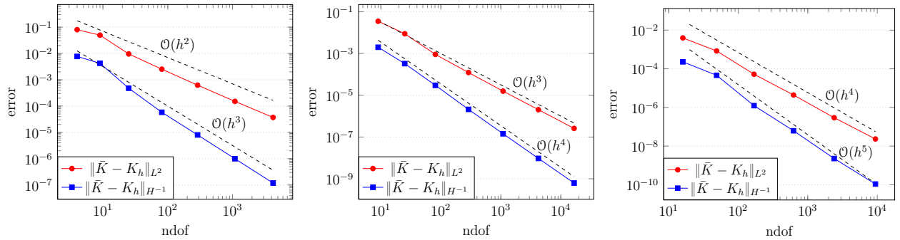
FIGURE 2. Convergence of pure lifted Gauss curvature with respect to number of degrees of freedom (ndof) in different norms for Regge elements g_h \in \text{Reg}_h^k of order k = 1, 2, 3 .
