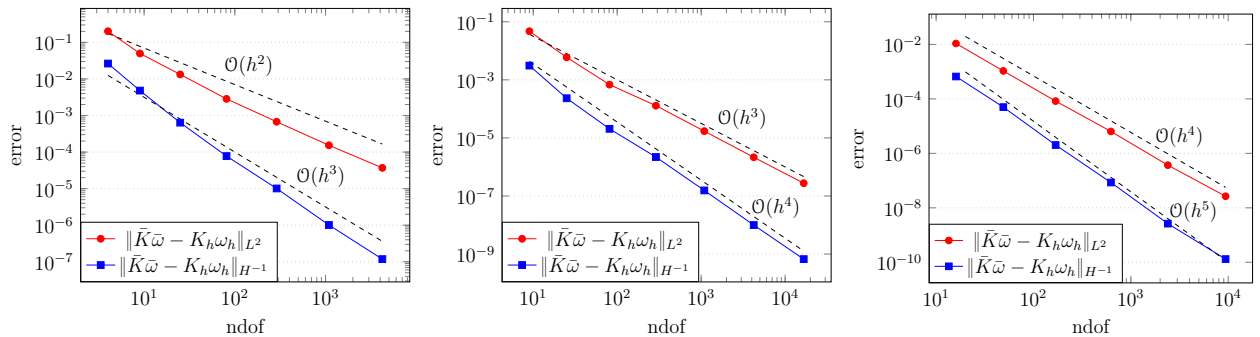
FIGURE 1. Convergence of lifted densitized Gauss curvature with respect to number of degrees of freedom (ndof) in different norms for Regge elements g_h \in \text{Reg}_h^k of order k = 1, 2, 3 .
