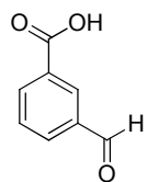
3-formylbenzoic acid
