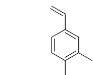
1,2-dimethyl-4-vinylbenzene
