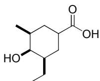
(3R,4S,5S)-3-ethyl-4-hydroxy-5-methylcyclohexanecarboxylic acid
