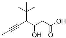
(3R,4R)-4-( tert -butyl)-3-hydroxyhept-5-ynoic acid
