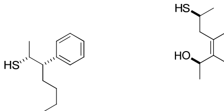
(2R,3S)-3-phenylheptane-2-thiol
