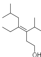
(Z)-4-ethyl-3-isopropyl-6-methylhept-3-en-1-ol
