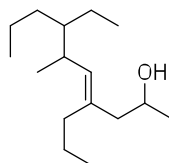
(E)-7-ethyl-6-methyl-4-propyldec-4-en-2-ol
