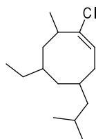
(E)-1-chloro-6-ethyl-4-isobutyl-8-methylcyclooct-1-ene
