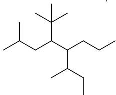
4-( tert -butyl)-2,6-dimethyl-5-propyloctane
