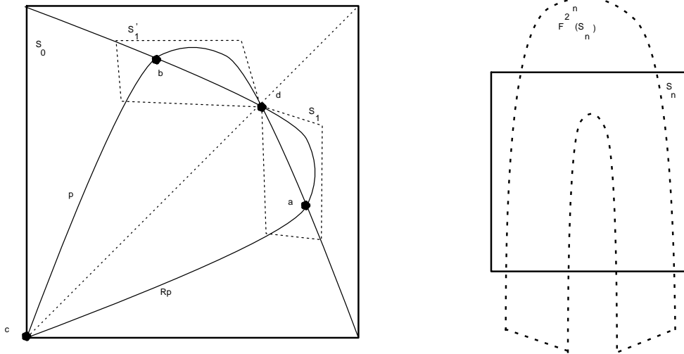
Figure 0.1: In a) the boxes S_0 and S_1 , the fixed points and points of period 2 are drawn. In b) the S_i and its image F^{2^i}(S_i) .
