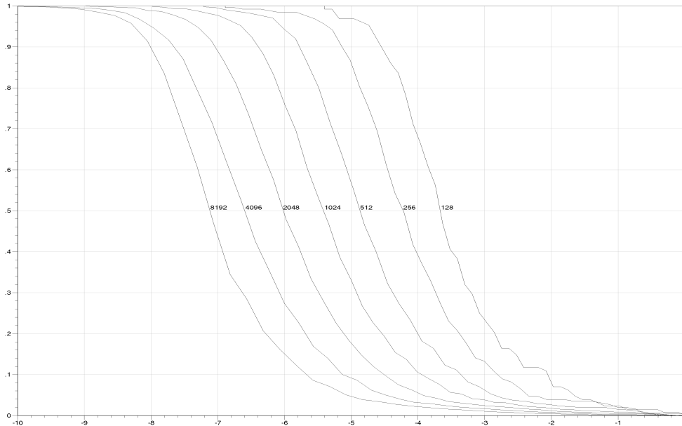
Figure 0.2: The curves are the distribution functions for scalings in error > 10^{-n} , -n the abscissa, for intervals of the labeled number of iterations. (Magnify to obtain a more accurate rendering).
