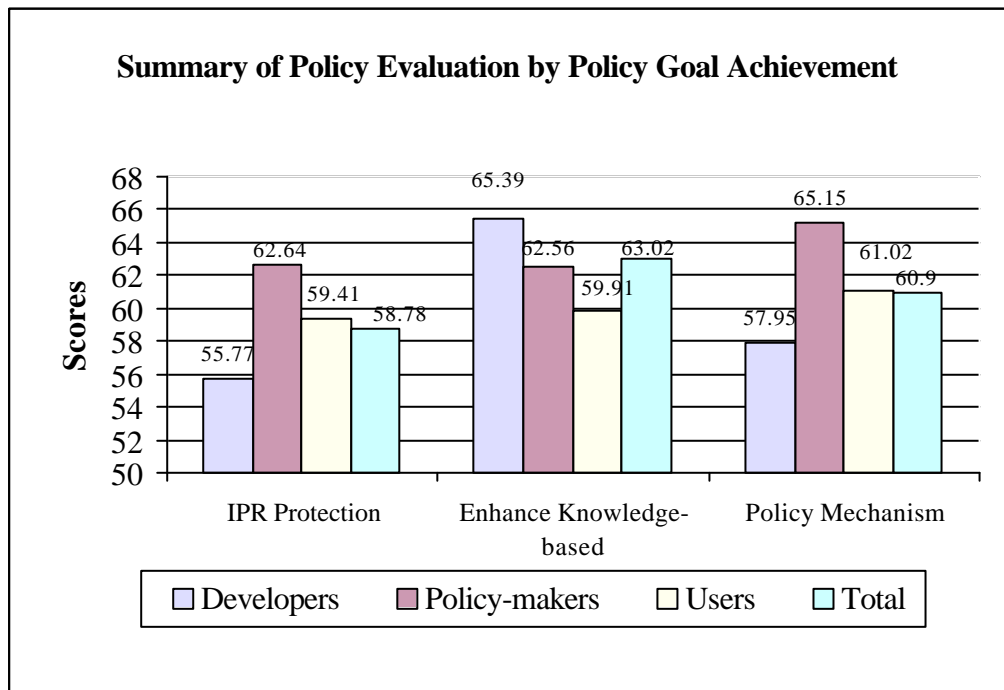
Figure 4 Policy Evaluation with MAUT Separated by Existing and Future Evaluation
