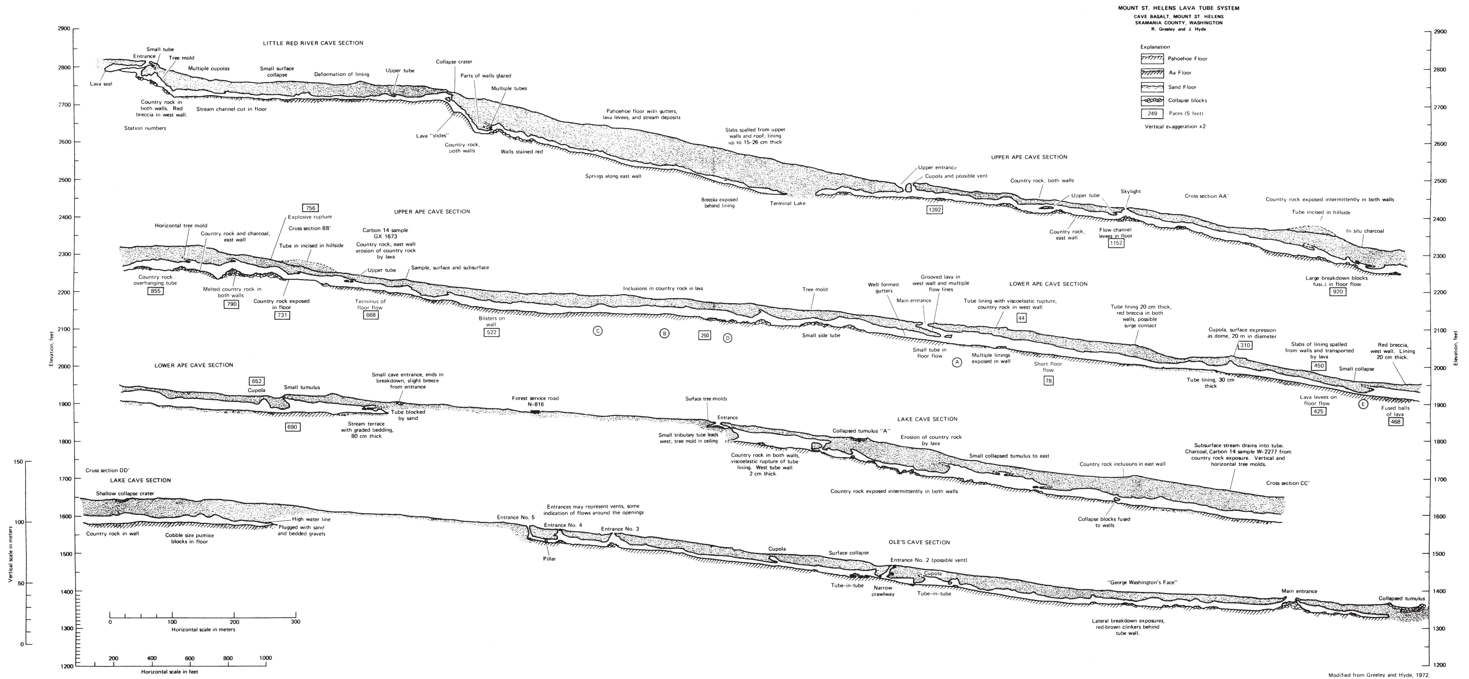
Figure 10. Longitudinal profiles of Mount St. Helens lava tubes.
