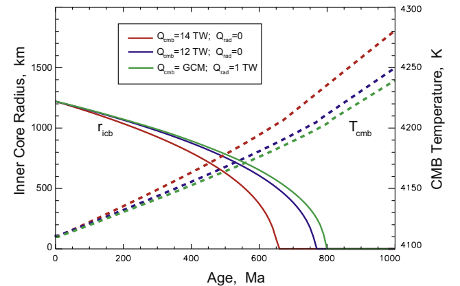
Fig. 6. Evolution of the core for different values of the total CMB heat flow, assumed constant in time. T_{cmb} and r_{icb} denote CMB temperature and inner core radius, respectively.
