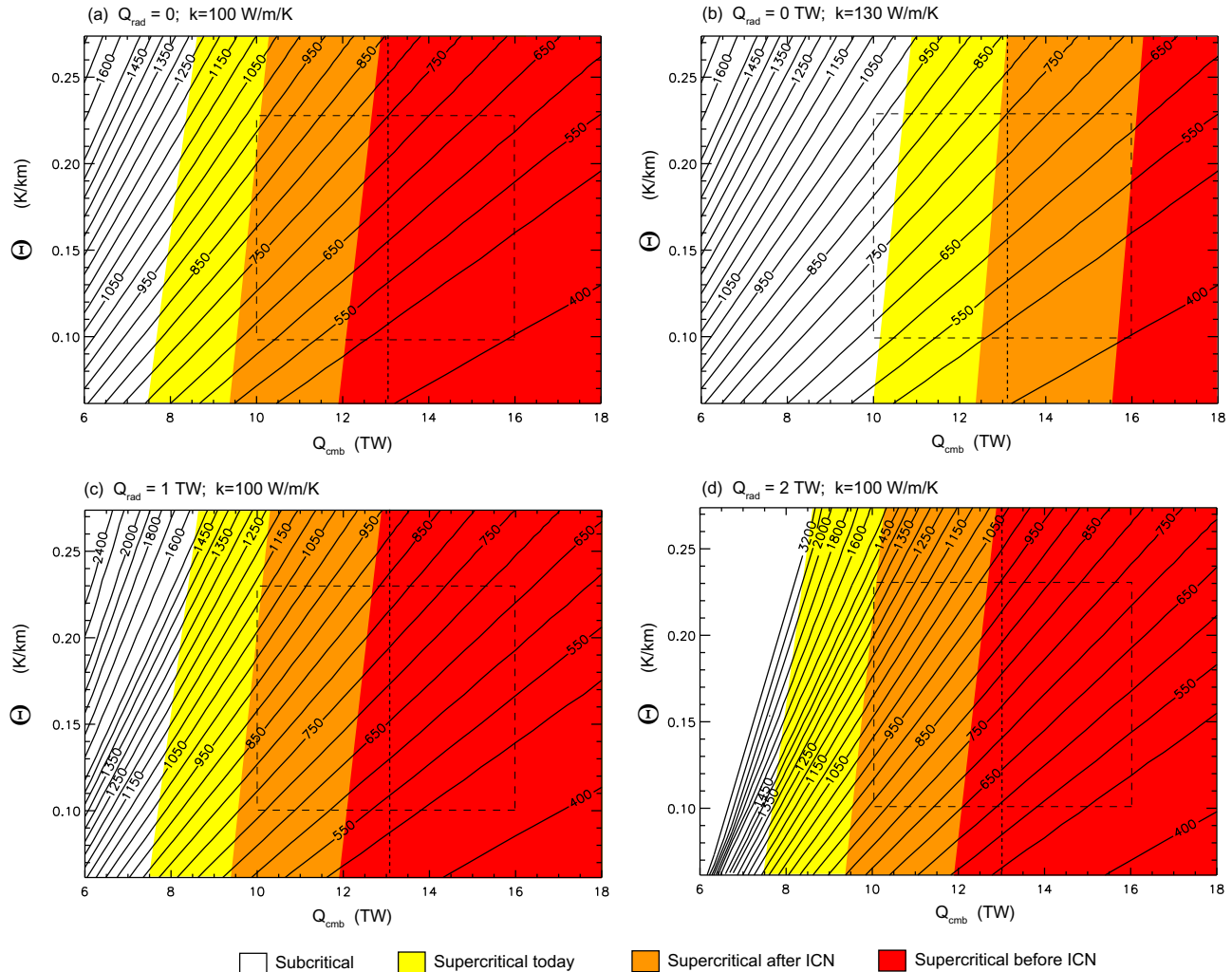
Fig. 7. Predicted ages of inner core nucleation (ICN) in millions of years as a function of total CMB heat flow Q_{\text{cmb}} and \Theta , the difference between the slope of the melting curve and the adiabat at the inner core boundary, calculated using different combinations of present-day potassium-40 radioactive heat production Q_{\text{rad}} and outer core thermal conductivity k . Panels a, c, and d use k = 100 \text{ W m}^{-1} \text{ K}^{-1} ; panel b uses k = 130 \text{ W m}^{-1} \text{ K}^{-1} ; top row (a and b) use Q_{\text{rad}} = 0 ; bottom row: (c and d) use Q_{\text{rad}} = (1, 2) \text{ TW} , respectively. Shadings correspond to dynamo states: white = subcritical; yellow = supercritical today; light brown = supercritical 50 Myr after ICN; red = supercritical just prior to ICN. Dashed boxes indicate allowed region based on mantle GCMs and core melting relations. Dotted lines indicate the time average Q_{\text{cmb}} from our mantle GCMs. (For interpretation of the references to colour in this figure legend, the reader is referred to the web version of this article.)
