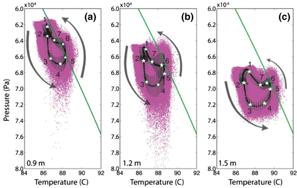
Fig. 8. Water pressure and temperature during the eruption cycles, for ~3531 eruptions. Gray arrows show the evolution of pressure and temperature with respect to time (stars 1 through 7: t_1 = 0 s, t_2 = 65 \pm 2 s, t_3 = 70 \pm 2 s, t_4 = 85 \pm 2 s, t_5 = 100 \pm 2 s, t_6 = 105 \pm 2 s, t_7 = 120 \pm 2 s). Black curves show the average and the black bars show the standard deviation of the data. Green lines show the calculated boiling curve for pure water.
