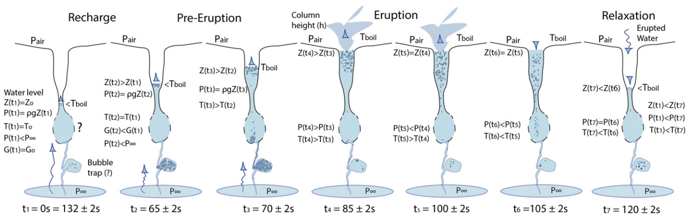
Fig. 14. Conceptual model for El Jefe geyser showing the different stages of the eruption cycle: recharge, pre-eruption, eruption, and relaxation. The model includes a bubble trap or cavity adding steam to the conduit. Blue dots inside the conduit represent bubbles of steam. Blue background represents liquid water. Conditions of pressure ( P ), temperature ( T ), water level ( Z ), and mass flow ( G ) inside the conduit evolve with time. The progression from t_1 to t_7 corresponds to the key stages in the cycle (Fig. 3).
