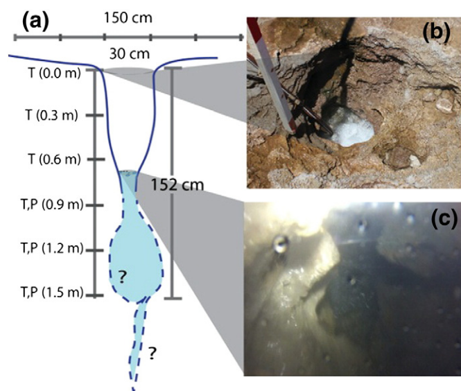
Fig. 2. (a) Illustration of the conduit and the locations of the deployed temperature (T) and pressure (P) sensors. (b) Photograph of the conduit mouth, while the water level was decreasing, showing the string of sensors; distance between the red marks is 30 cm. (c) Photograph of the conduit at the air–water interface (0.6 m) showing the irregular conduit, with constrictions and cracks that intersect the conduit.
