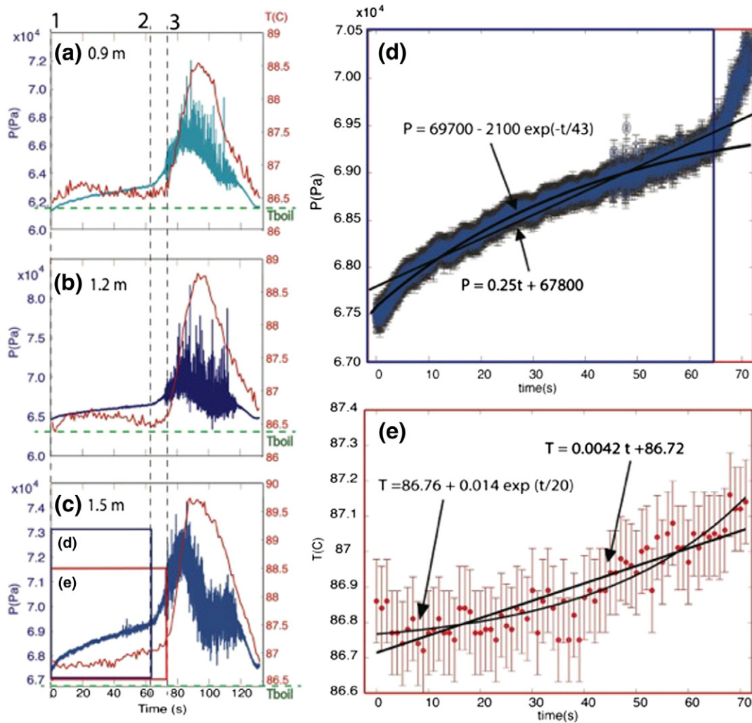
Fig. 11. Data from sensors located at (a) 0.9 m, (b) 1.2 m, and (c) 1.5 m. Pressure (blue) and temperature (red) data on the y-axes, and time for a single eruption cycle on the x-axis. Green line shows the boiling temperature at atmospheric conditions T_{\text{boil}} (86.4 °C). Numbers 1, 2 and 3 are the same key points described in previous figures. (d) Shows the pressure during the resting time. Fitting curves of the data are the black lines, and vertical gray lines show \pm 1 standard deviation. (e) Temperature during the same period. Fitting curves are the black lines, and the red vertical lines show \pm 1 standard deviation.
