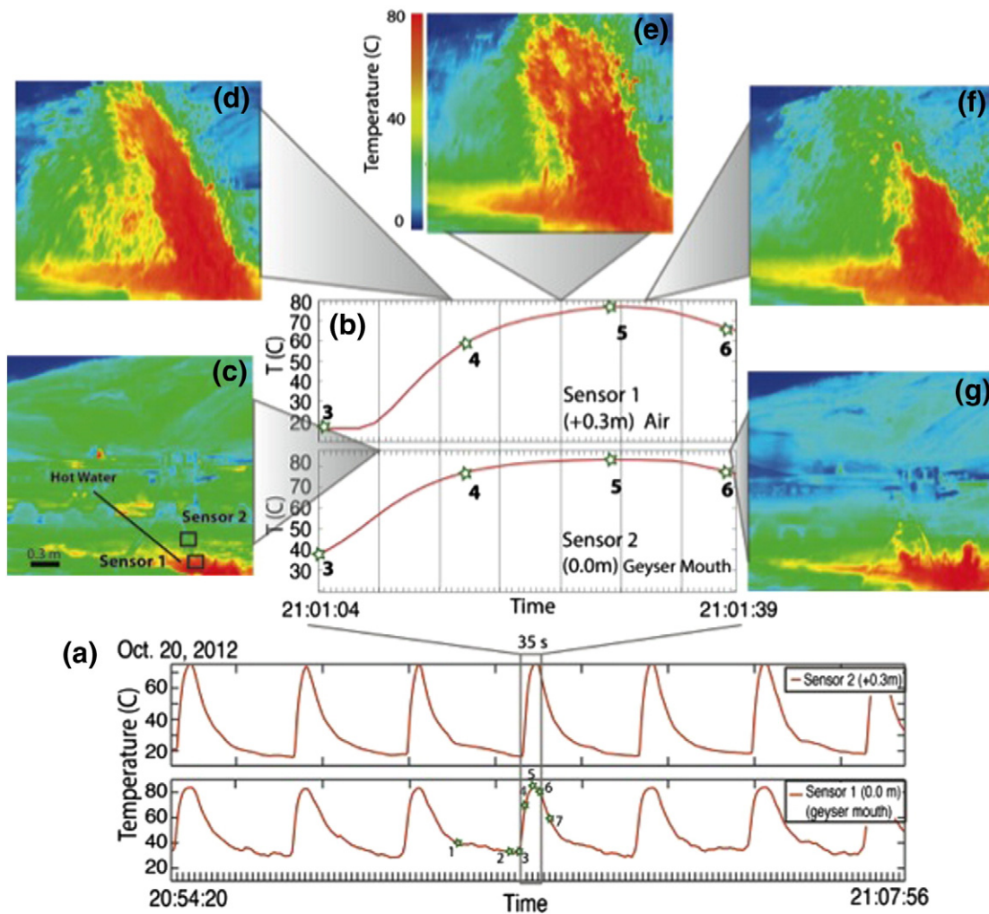
Fig. 5. (a) A sub-sample of the temperature time series for two sensors at the surface. Every peak represents an eruption. Sensor 1 is located at the geyser mouth. Sensor 2 is located 0.3 m above the conduit mouth. Sensors were in the air before eruptions occur. During the eruption, temperature increased because hot erupted water reached the sensors. (b) Zoom on 35 s of a single eruption (box). Stars with numbers are the key stages in the eruption cycle defined in Fig. 3, but for a different eruption. Images (c) to (g) were taken with a FLIR camera (extracted from the video every ~6 s) during the same eruption. High temperature, in red, is related to boiling water coming out of the conduit during the eruption. Image (c) was taken shortly after the start of the eruption at point 3, and it shows the high temperature in the mouth of the conduit. Between points 4 and 6, temperature remains close to T_{\text{boil}} , the boiling point; subsequent images (d), (e), and (f) show a high volume of hot water coming out of the conduit. At point 6, temperature decreases (sensor in contact with air). The volume of hot water drops (image (g)) identifying the end of the eruption at the surface.
