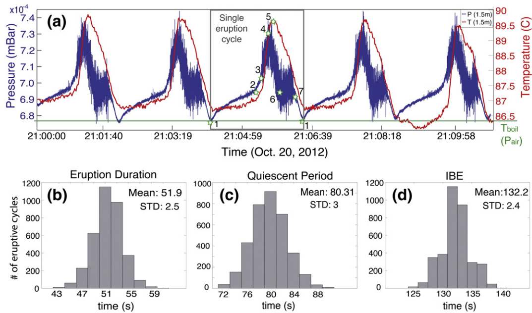
Fig. 3. a) Pressure and temperature time series for a subset of five eruption cycles, at a depth of 1.5 m, on October 20th, 2012. Temperature (red) and pressure (blue) data are plotted on the y-axis, while time is on the x-axis. The box highlights a single cycle. Stars labeled from 1 to 7 identify key stages in the cycle. The green line shows mean boiling temperature ( T_{\text{boil}} \sim 86.4^\circ\text{C} ) at average local atmospheric pressure. Lower panel shows histograms of the duration of stages of the eruption cycles: (b) eruption duration (points 3 to 7), (c) quiescent period (including relaxation stage, recharge, and pre-eruptive stage, points 7 to 3), and (d) interval between eruptions (IBE).
