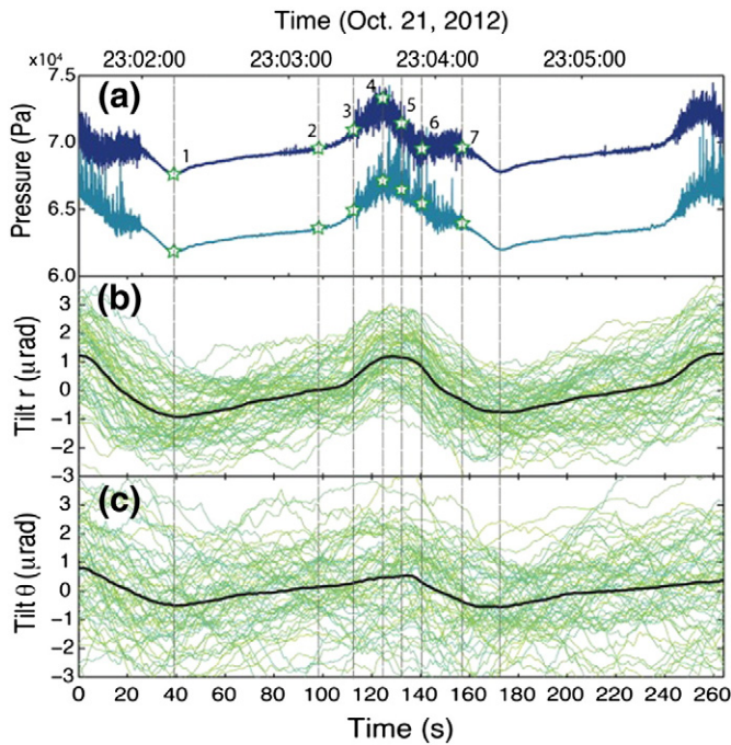
Fig. 6. (a) The pressure measured at depths of 1.5 m (dark blue) and 0.9 m (light blue). (b) and (c) show the ground deformation recorded by a tiltmeter, in the radial and tangential directions, respectively. A positive sign indicates that the ground rises in the direction of vent and to the north, respectively. Black curves are the averaged signals. Yellowish to bluish curves are for individual eruptions.
