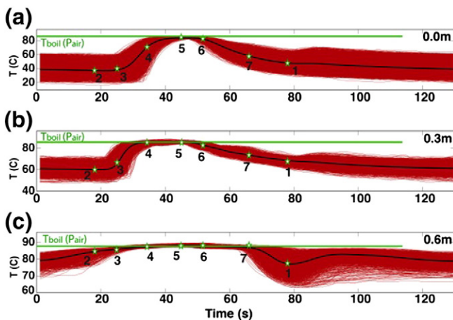
Fig. 7. Temperature in the shallowest part of the conduit for 3531 geyser cycles at depths of (a) 0.0 m, (b) 0.3 m, and (c) 0.6 m. The geyser cycles (red curves) are stacked and averaged (black curves). Range of time is the IBE (132 s). The green line shows the boiling temperature ( T_{\text{boil}} ) for the corresponding air pressure ( P_{\text{air}} ). From points 2 to 3, the temperature increases. After point 3, water reaches the boiling curve at 0.6 m, and the eruption starts. Between points 4 and 5, boiling water reaches the shallowest sensors at 0.3 m and 0.0 m. Between points 6 and 7, water continues to boil at 0.6 m, but boiling water does not reach the shallowest sensors and the eruption ends at the surface. At point 1, cooled erupted water returns to the conduit and the cycle starts again.
