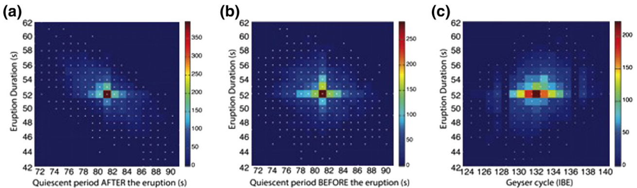
Fig. 9. 2-D histograms of (a) relationship between eruption duration and duration of following quiescent period, the coefficient of correlation is r^2 = 0.4 ; (b) relationship between eruption duration and duration of previous quiescent period, the coefficient of correlation is r^2 = 0.03 (c) Relationship between eruption duration and IBE, the coefficient of correlation is r^2 = 0.06 . IBE is defined for an entire geyser cycle: the period between the beginning of an eruption and the beginning of the next eruption (eruption duration plus the quiescent period after eruption). White dots show the data, and colors show the number of observations plotting in that region (color bar).
