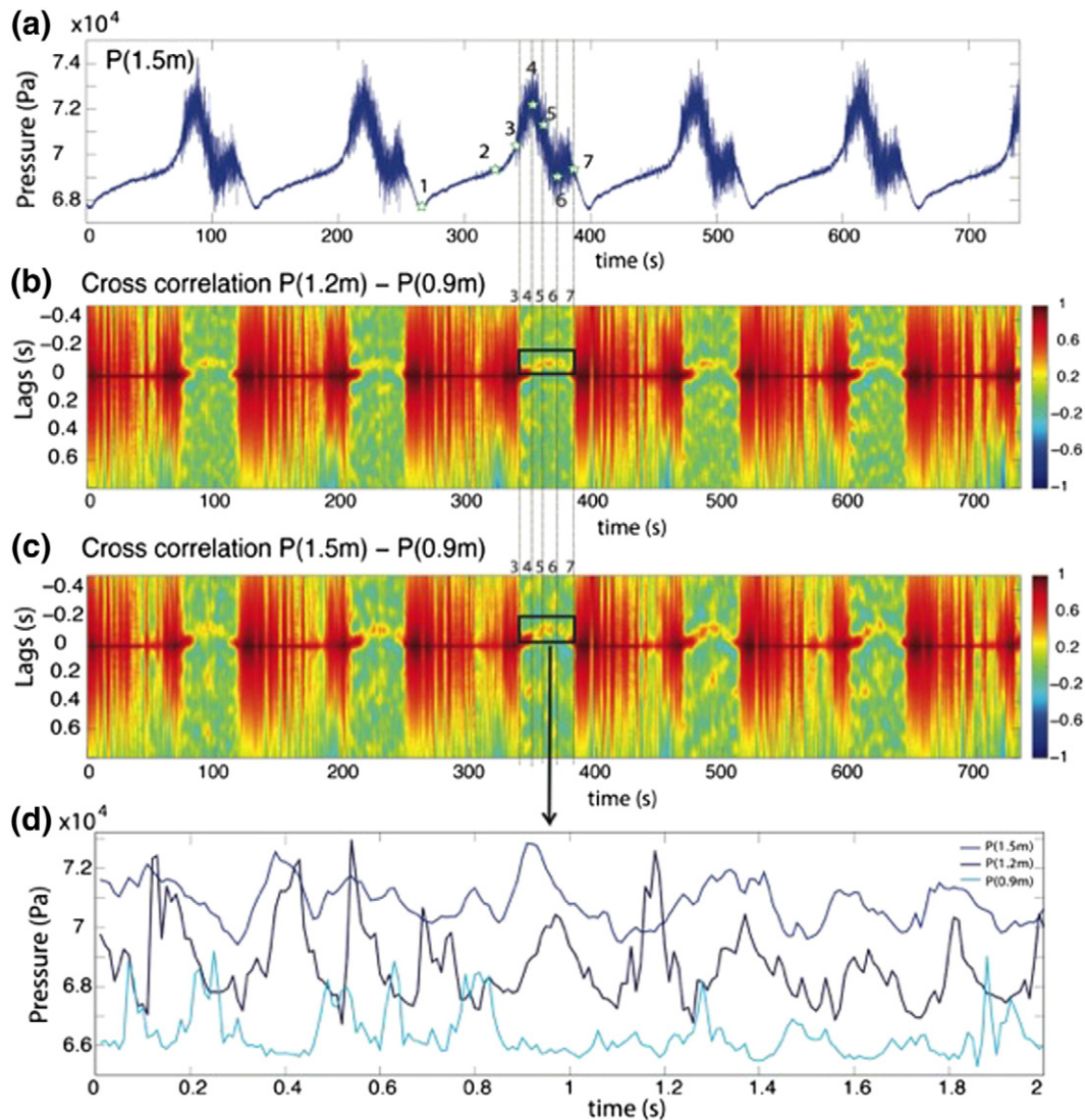
Fig. 13. (a) Pressure data of a subsample of five eruptions from a sensor located at a depth of 1.5 m. Plots (b) and (c) show the cross-correlation between pressure data from different depths. Time is shown on the horizontal axis and the vertical axis shows the time lag (in seconds) for the cross-correlation. (b) Cross-correlation of sensors located at 1.2 m and 0.9 m, showing a strong cross-correlation at a time lag of -0.1 s (black box). The negative lag means that the signal arrives first at 1.2 m and then at 0.9 m, propagating upward with a speed of 3 m/s. (c) Cross-correlation between sensors located at 1.5 m and 0.9 m, showing a strong signal at -0.15 s (black box). The pressure signal is moving upward with a speed of 4 m/s. (d) Pressure data subsample of 2 s during the eruption.
