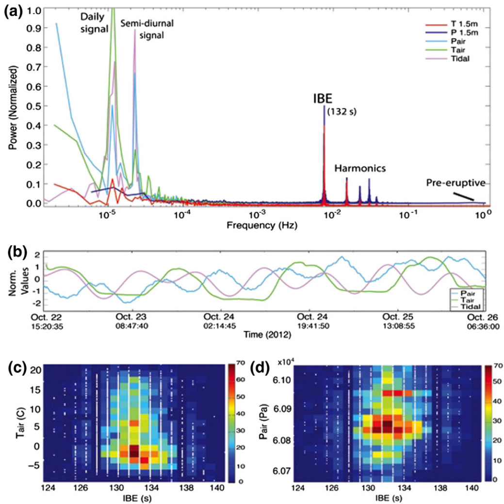
Fig. 4. (a) Power spectra of pressure (blue) and temperature (red) inside the geyser (1.5 m), and external periodic daily signals: air temperature ( T_{\text{air}} ), atmospheric pressure ( P_{\text{air}} ), and calculated solid Earth tides (Tidal). Values on the y-axis were normalized to have the same scale. One day period observed in the water temperature (1.5 m) data is an instrumental artifact and not a real signal. (b) Time series for 3.5 days showing daily variations of air temperature, atmospheric pressure and solid Earth tides. Values shown on y-axis were normalized ((Value – mean(Value)) / Std(Value)). (c) and (d) are 2-D histograms: white dots show the data, and colors show number of dots plotting in that region (color bar). (c) IBE as a function of air temperature, the coefficient of correlation is r^2 = 0.01 (d) IBE as a function of atmospheric pressure, the coefficient of correlation is r^2 = 0.02 .
