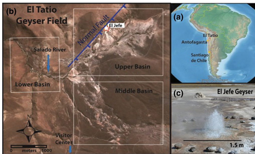
Fig. 1. El Tatio geyser field. (a) Map of South America showing the location of El Tatio in Northern Chile. (b) Aerial photograph of El Tatio Geyser Field (GLCF: Earth Science Data Interface); white boxes show the Upper, Middle, and Lower geyser basins. In the upper basin, El Jefe Geyser (UTM coordinates 601768 E; 7530174 S, WGS84, 19S) is marked by the white star. The blue line indicates the normal fault that bounds the El Tatio half-graben. El Jefe geyser is located in the hanging wall of that fault. (c) El Jefe geyser erupting.
