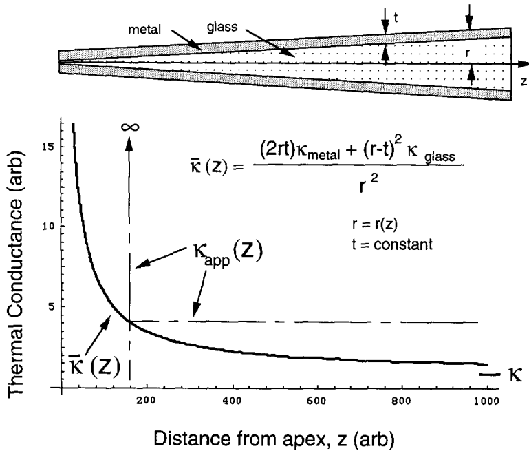
Fig. 3. Thermal conductance of a probe as a function of distance from probe apex (solid curve). The conductance falls as the fraction of (relatively high conductivity) Al decreases while that of (relatively low conductivity) glass increases. To model the behavior of thermal diffusion, the dash-dotted profile was chosen. Near the apex, conductance is assumed to be infinite, while at larger distances ( z > z_c = 160 arbitrary units) a value approximately three times the value at z = \infty is chosen.
