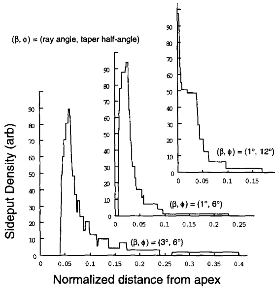
Fig. 2. Sideput density versus distance from the apex for a number of conical probes for a variety of (\beta, \phi) values (given in degrees). While the plots differ somewhat, common to all is an indication of a large sideput density well removed from the taper apex.
