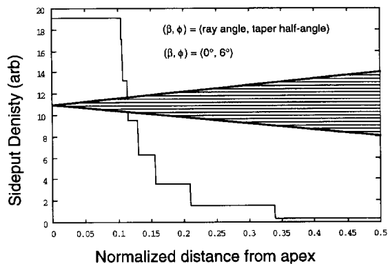
Fig. 1. The sideput density for a conical probe. A bundle of rays of half-angle \phi = 6^\circ that diverge from being co-axial by an angle \beta = 0^\circ and that fills the conical taper is shown across the middle of the figure. The sideput density plot represents a measure of the interactions of the bundle of rays with the reflecting walls of the cone. The interactions can be tracked by following the image of the trajectory in the repeated zones.
