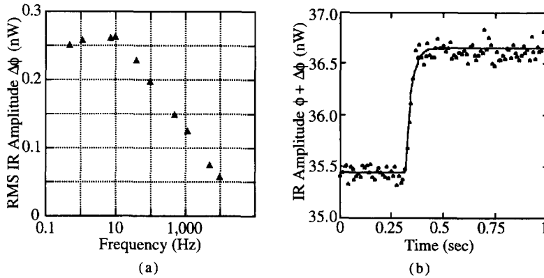
Fig. 4. Temporal response of a typical probe to a rapid 0.6 mW pulse of visible radiation as monitored by a 0.35 mW input of CW IR light. The infrared signal as a function of time is plotted at the right of the figure. The data fit a single exponential decay of \tau = 0.02 s quite well. The infrared signal as a function of frequency \nu is shown at the left of the figure. Within the precision of the measurement \nu_{\text{knee}} = 1/(2\pi\tau) .
