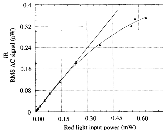
Fig. 6. Intensity dependence of the modulation of the infrared signal as a function of the input intensity. The intensity of the CW infrared light is held constant. At low intensities, linear scaling of the modulation with intensity suggests that neither the heat dissipation mechanism nor the thermal/optical coupling balance changes with intensity in this region.
