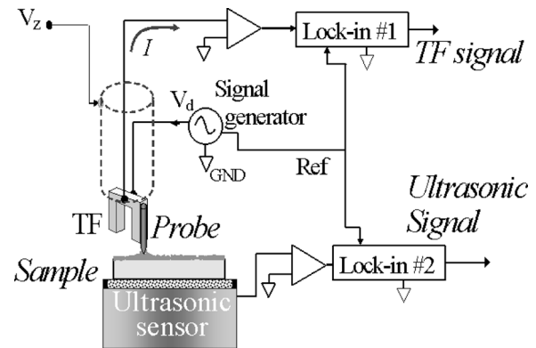
FIG. 1. Experimental setup for simultaneous measurement of the tuning fork and ultrasonic signals.
