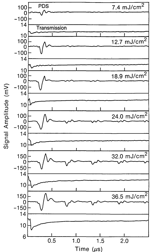
Fig. 3. Same as in Fig. 2 for the \alpha -Si sample in H_2O . PDS, photoacoustic deflection signal.
