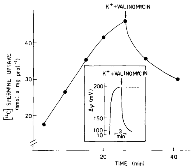
FIG. 3. Effect of \text{K}^+ + valinomycin on spermine uptake and \Delta\Psi . Mitochondria were incubated in the standard medium containing 1 mM [ ^{14}\text{C} ]spermine and 1 mM \text{P}_i . At 25 min, 10 mM KCl and valinomycin (0.33 \mu\text{g}/\text{mg} ) were added.
