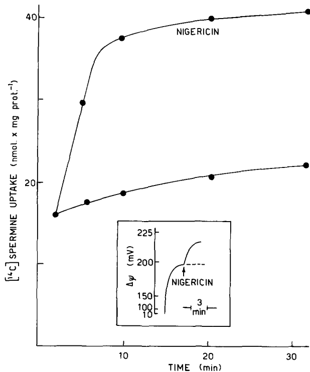
FIG. 2. Effect of nigericin on spermine uptake and \Delta\Psi . Mitochondria were incubated in the standard medium containing 1 mM [ ^{14}\text{C} ]spermine. When present, nigericin (0.33 \mu\text{g}/\text{mg} ) was added.
