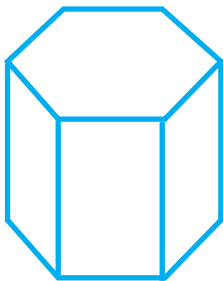
simplest, faceted crystal (plates, columns)
