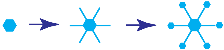
more complicated shapes
