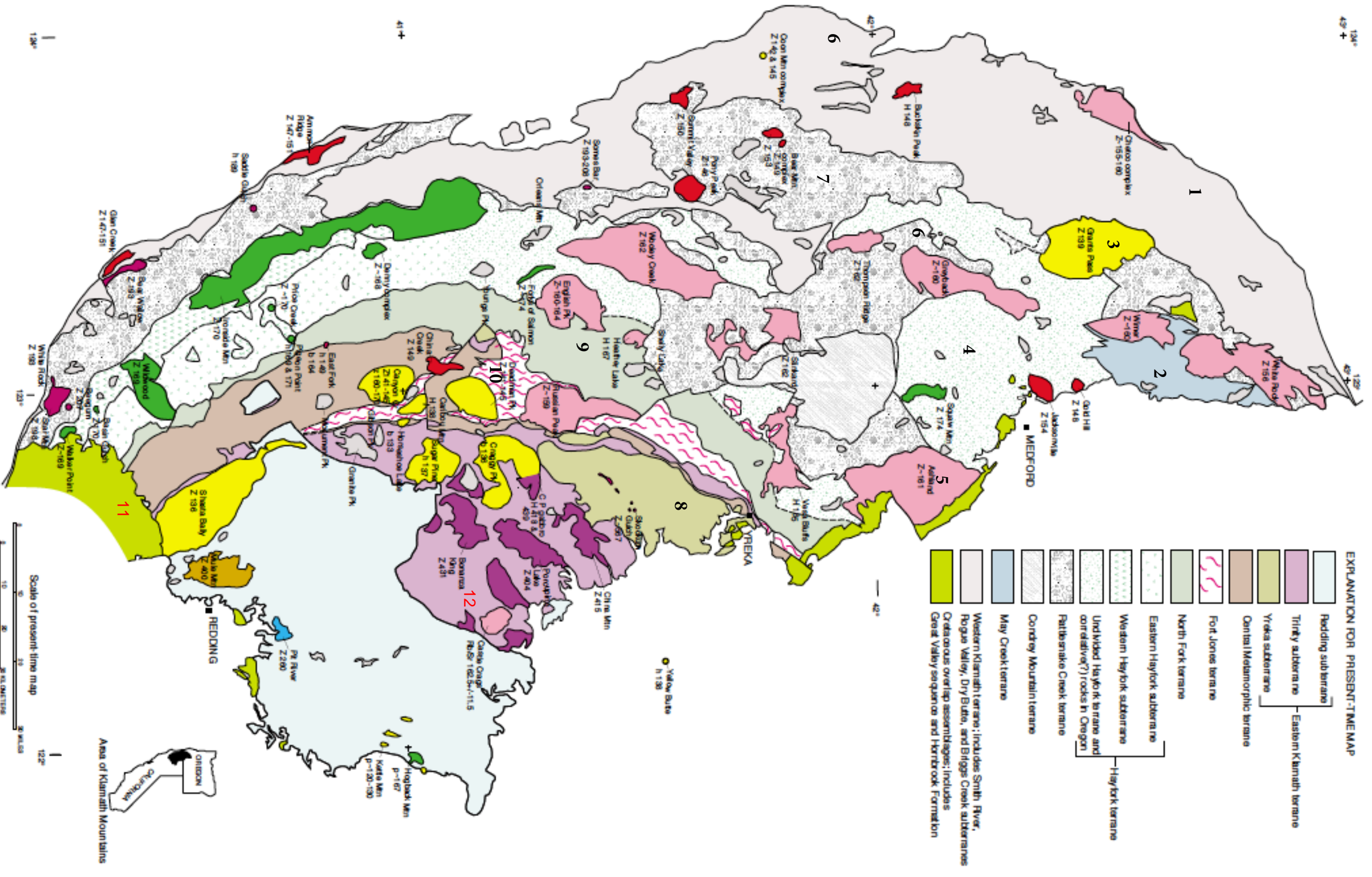
Figure 9 Present time Geology modified from Irwin (1994)
