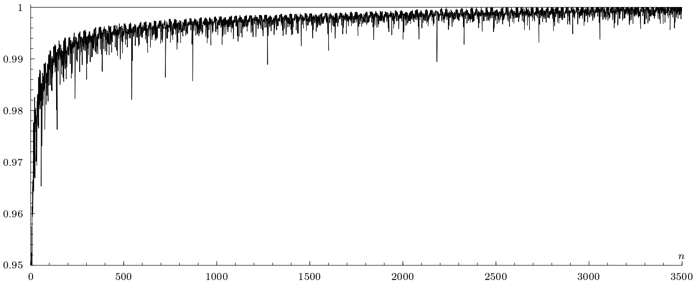
FIGURE 6. Dimension calculation when t \rightarrow 1/5 . The system is (3, \{0, 2+n, 9+5n\}) ; only the lower bound of the dimensions is given.
