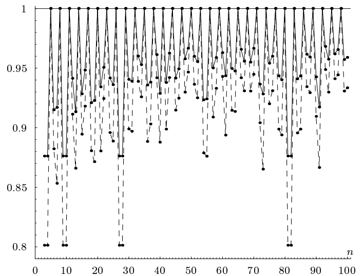
FIGURE 4. Dimension calculation when t \rightarrow 0 . The system is (3, \{0, 1, n\}) ; the upper (solid) curve gives the actual dimension, and the dashed curve gives the lower bound.
