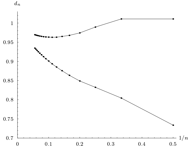
FIGURE 1. Direct calculation of the box dimension. Top curve: \log(N_n)/\log((3^n + 1)/2) . Bottom curve: \log(N_n)/(n \log 3) .
