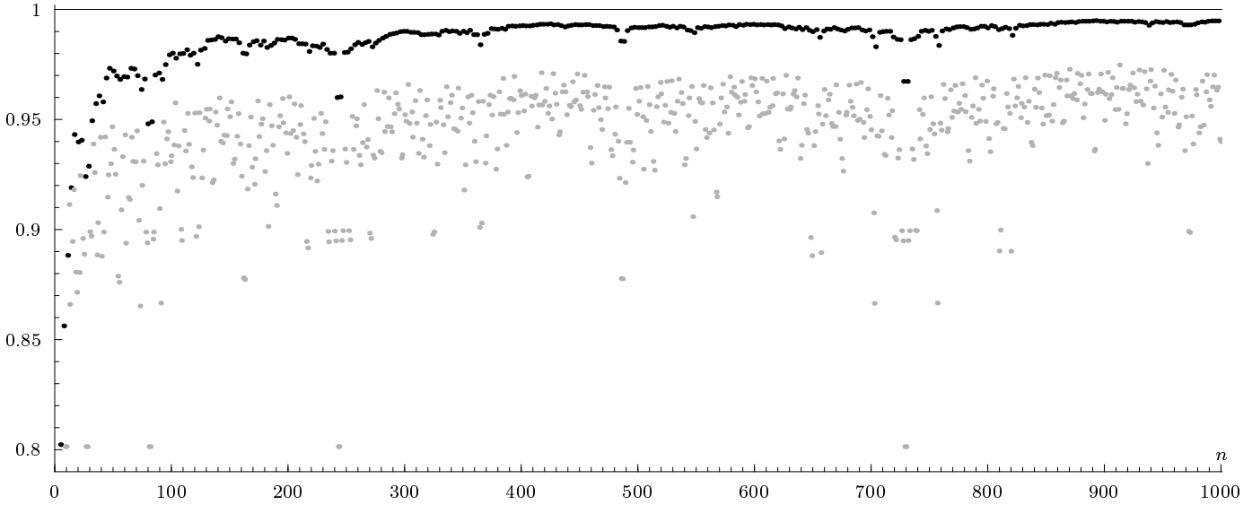
FIGURE 5. Dimension calculation when t \rightarrow 0 for large n . The system is (3, \{0, 1, n\}) ; the black dots give the dimension of the boundary, and the gray dots give the lower bound for the dimension. Not shown are the gray dots at (n, 1) for n = 2 \pmod 3 .
