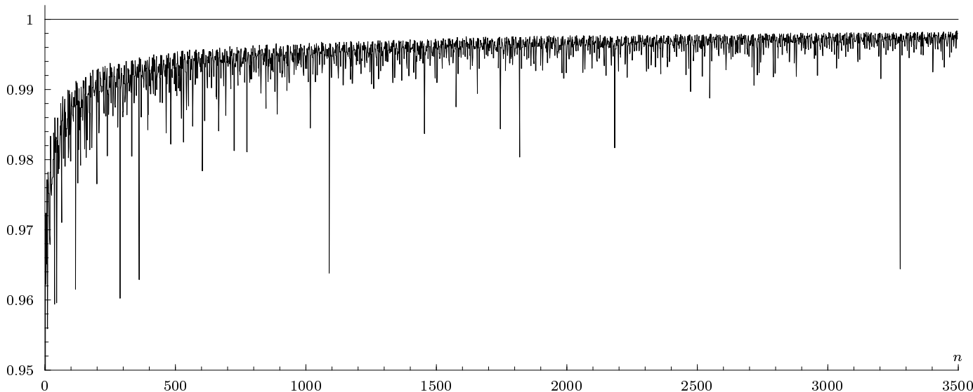
FIGURE 7. Dimension calculation when t \rightarrow 2/5 . The system is (3, \{0, 3+2n, 8+5n\}) ; only the lower bound of the dimensions is given. For clarity, those n where the value is 1 are not shown.
