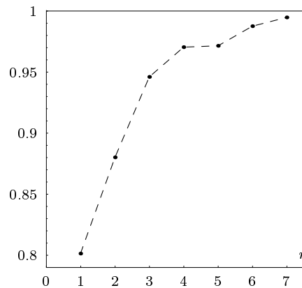
FIGURE 8. Dimension calculation when t approaches (\sqrt{13}-3)/2 . The system is (3, \{0, c_{n-1}, c_n\}) , where the c_i are defined in (4-2); the dots show the lower bound of the dimension.
