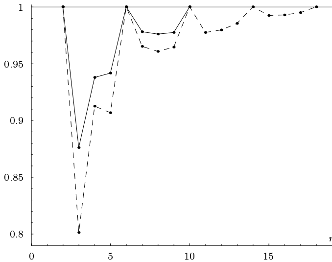
FIGURE 2. Dimension calculation when t \rightarrow g . The system is \{3, 0, f_{n-1}, f_n\} ; the solid curve gives the actual dimension, and the dashed curve the lower bound of the text.
