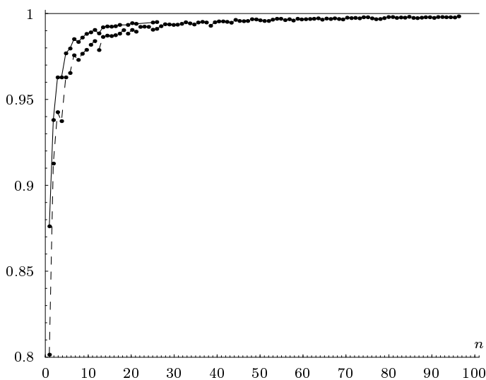
FIGURE 3. Dimension calculation when t \rightarrow 1/2 . The system is (3, \{0, n/(2n+1), 1\}) ; the upper (solid) curve gives the actual dimension, and the dashed curve that extends to the right gives the lower bound.
