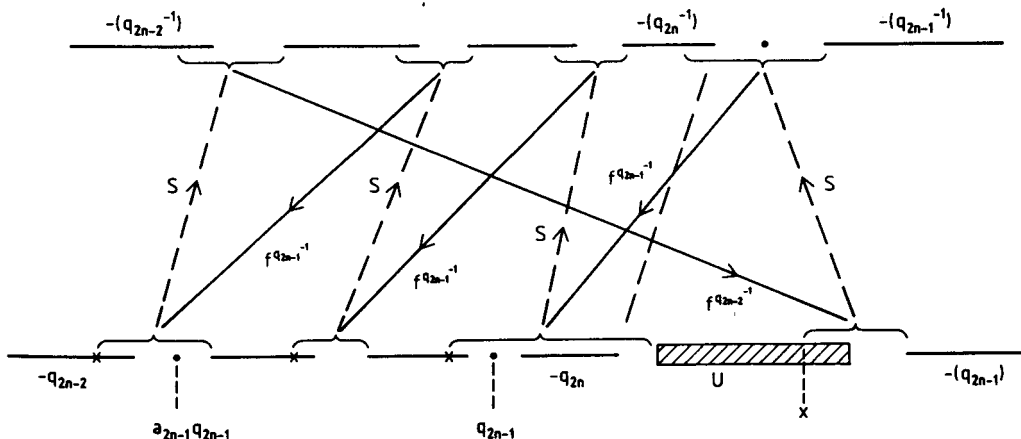
Fig. 7.1. Propagation of the scalings along an orbit
