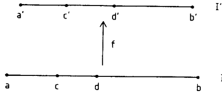
Fig. 3.1. Geometry of the Koebe principle
