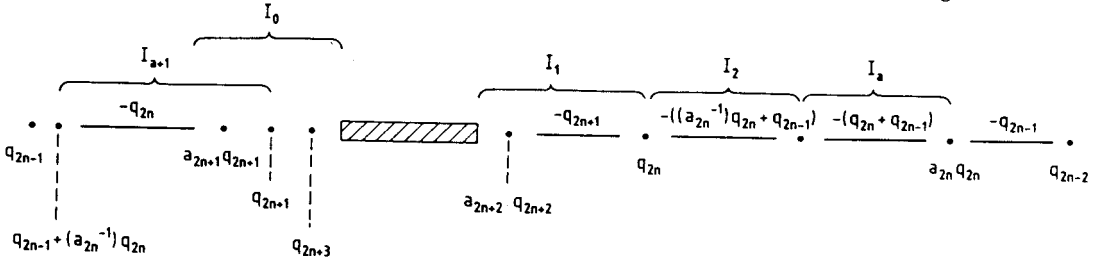
Fig. 4.1. The configuration for irrational number of the forward and backward orbit of the flat spot
