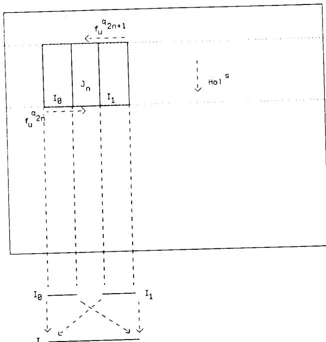
Fig. 5. Reduction to one-dimensional expanding maps.
