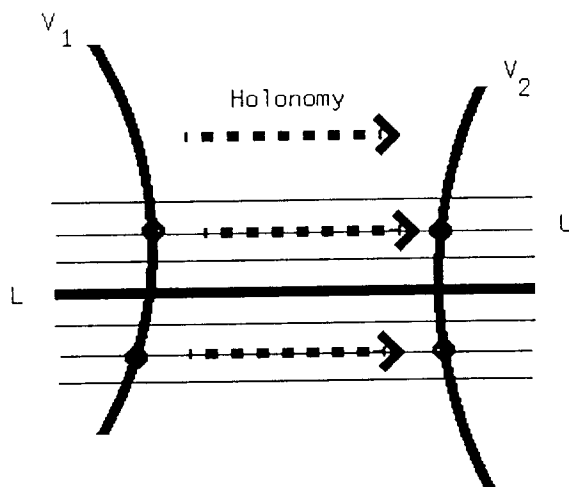
Fig. 3. The holonomy map: pushing along unstable leaves.
