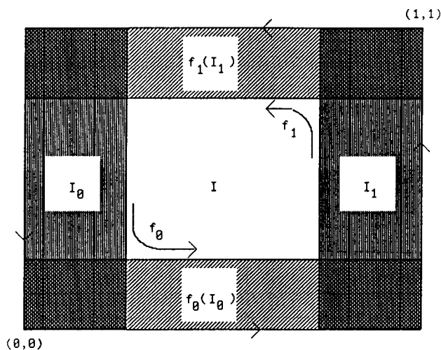
Fig. 2. The geometric definition of the maps f_0 and f_1 .
