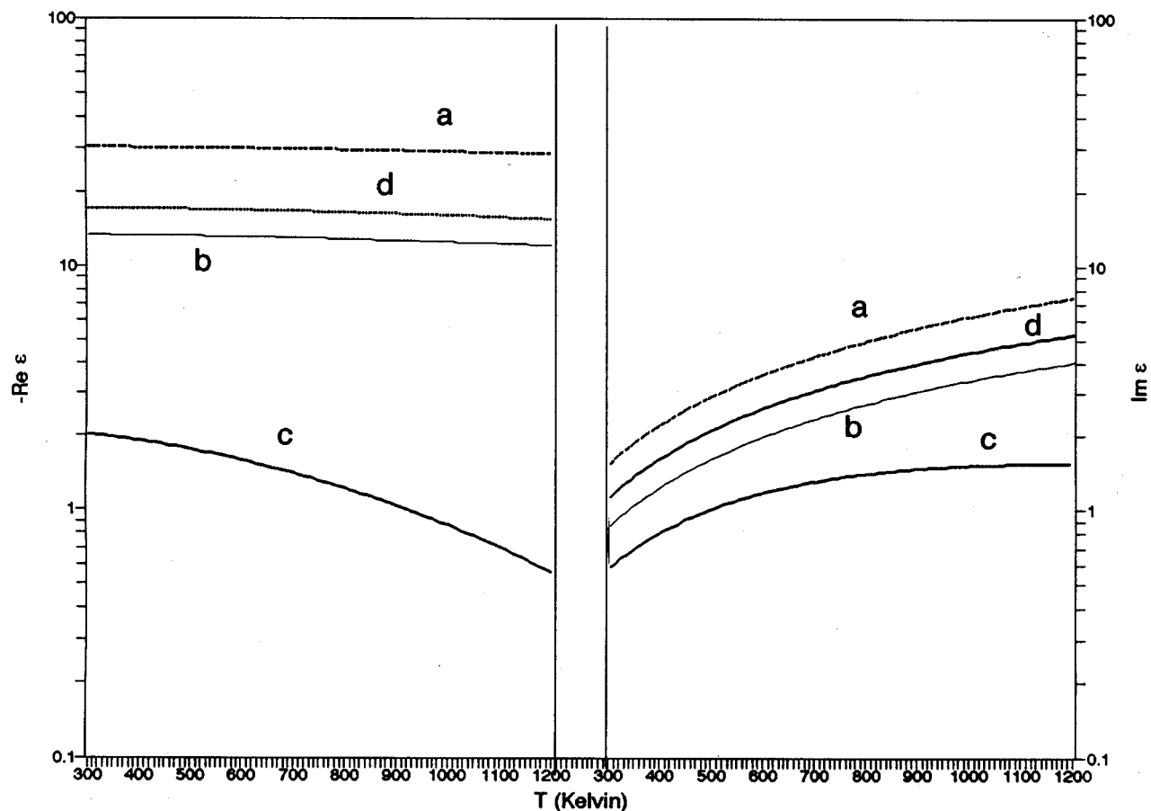
FIG. 5. The real and imaginary parts of the dielectric function for Ag as a function of temperature at different frequencies as labeled in Figs. 1 and 3.
